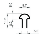
COR-4700 Stainless steel rail
