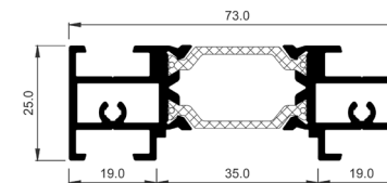
COR-3740 Adjustable jamb
