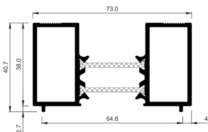
COR-3795 Frame supplement
