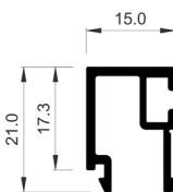
COR-3781 15 mm glazing bead
