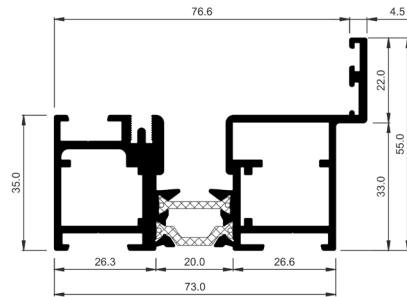
COR-3730 Frame with inox rail
