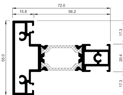
COR-3770 Sash transom
