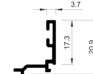
COR-3783 3,7 mm glazing bead
