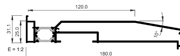
COR-3837 Subcill 180 mm
