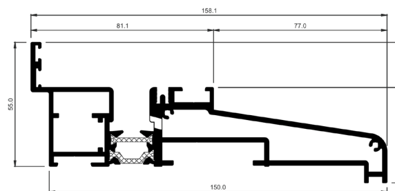
COR-3785 150 mm frame with drainage
