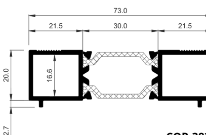
COR-3839 300 mm drainage subcill
