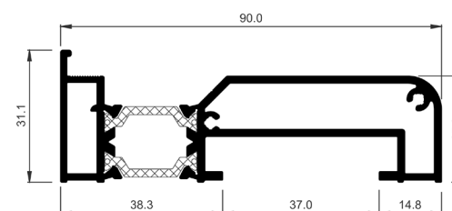
COR-3836 Subcill 90 mm
