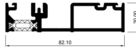
COR-3788 20 mm threshold with thermal break
