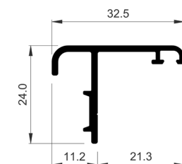
COR-3745 Swing door rebate
