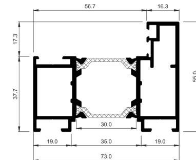
COR-3721 55 mm sash
