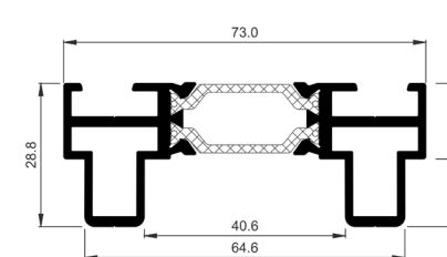
COR-3740 Adjustable jamb
