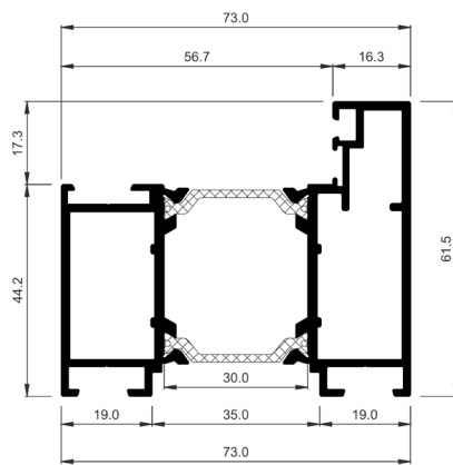
COR-3720 Standard sash
