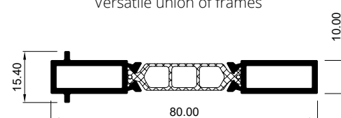
COR-3798 Versatile union of frames
