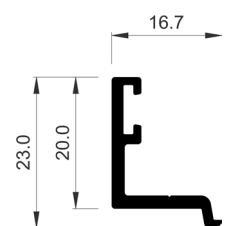
COR-3793 Swing door rebate for threshold
