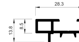
COR-3744 Half roller adapter
