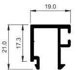
COR-3780 19 mm bead
