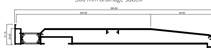
COR-3839 300 mm drainage subcill
