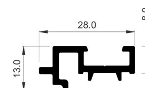
COR-3743 Swing door lock adaptor
