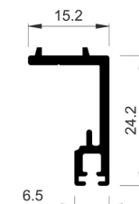
COR-3725 Sash extension
