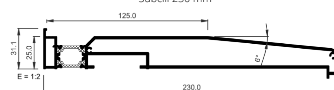
COR-3838 Subcill 230 mm
