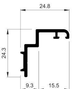
COR-3746 Swing door rebate
