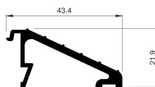
COR-3792 20 mm ramp for threshold
