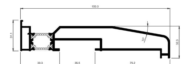
COR-3735 150 mm drainage subcill
