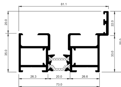
COR-3731 Lateral frame
