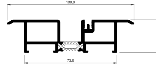
COR-3789 Threshold with thermal break
